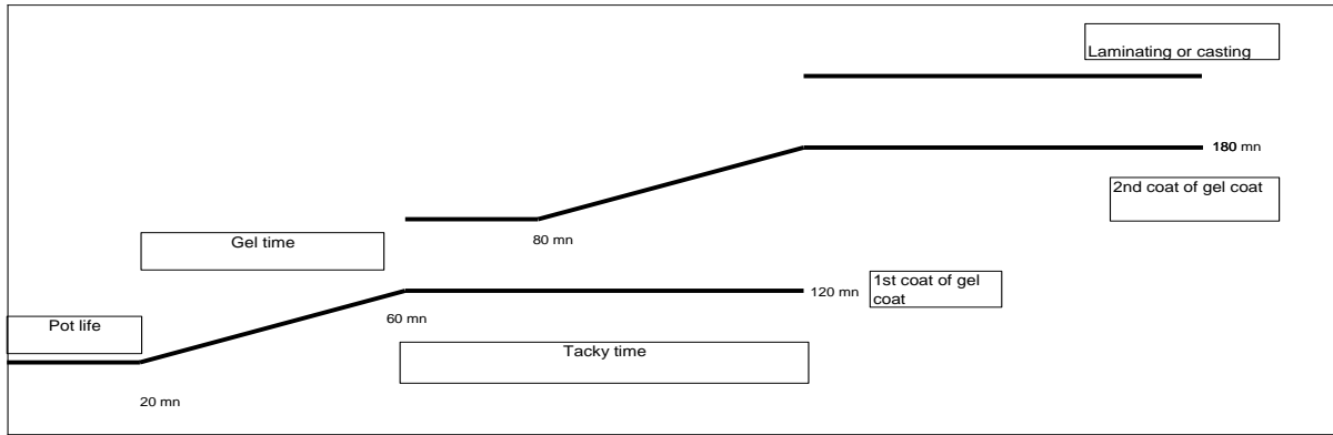
Application diagram of GC1 050 GN / GC 10 (Application temperature : 23°C Mass 500 g)
