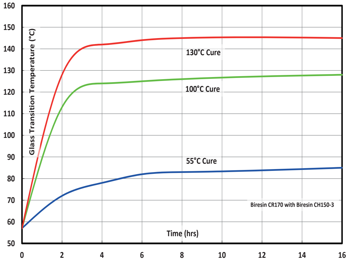
Glass Transition Temperature vs. Cure Cycle
